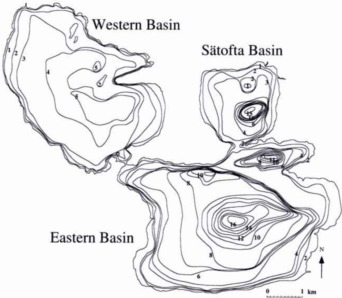
Figure 2. The three basins of Lake Ringsjön: Säftofta Basin, Eastern Basin and Western Basin. Depth contours for each meter are given.
